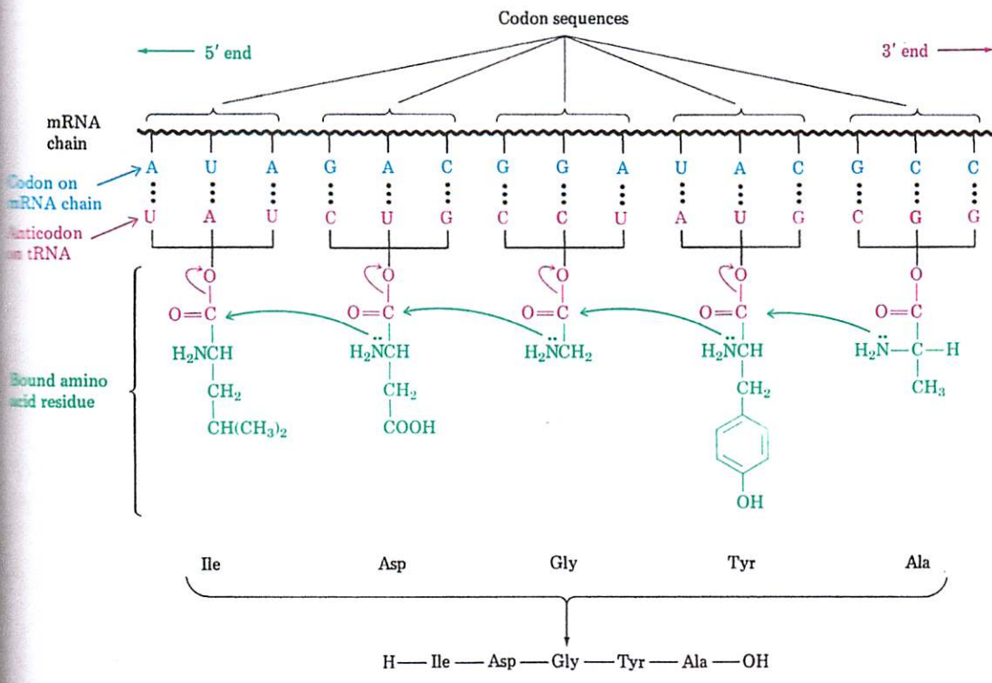
Figure 29.13 A schematic representation of protein biosynthesis. The mRNA containing codon base sequences is read by tRNA containing complementary anticodon base sequences. Transfer RNA assembles the proper amino acids into position for incorporation into the growing peptide.
