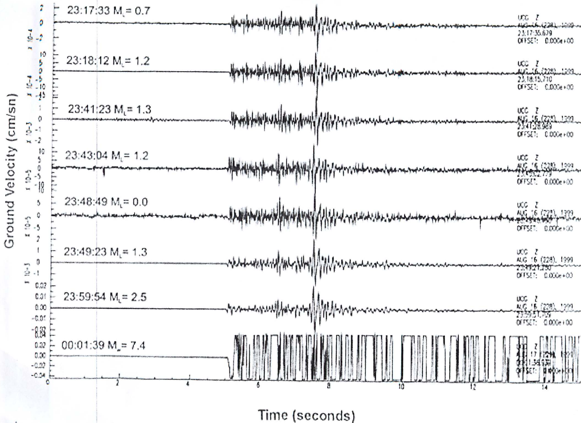
Figure 4. Seismograms of the foreshock sequence preceding the Izmit mainshock
