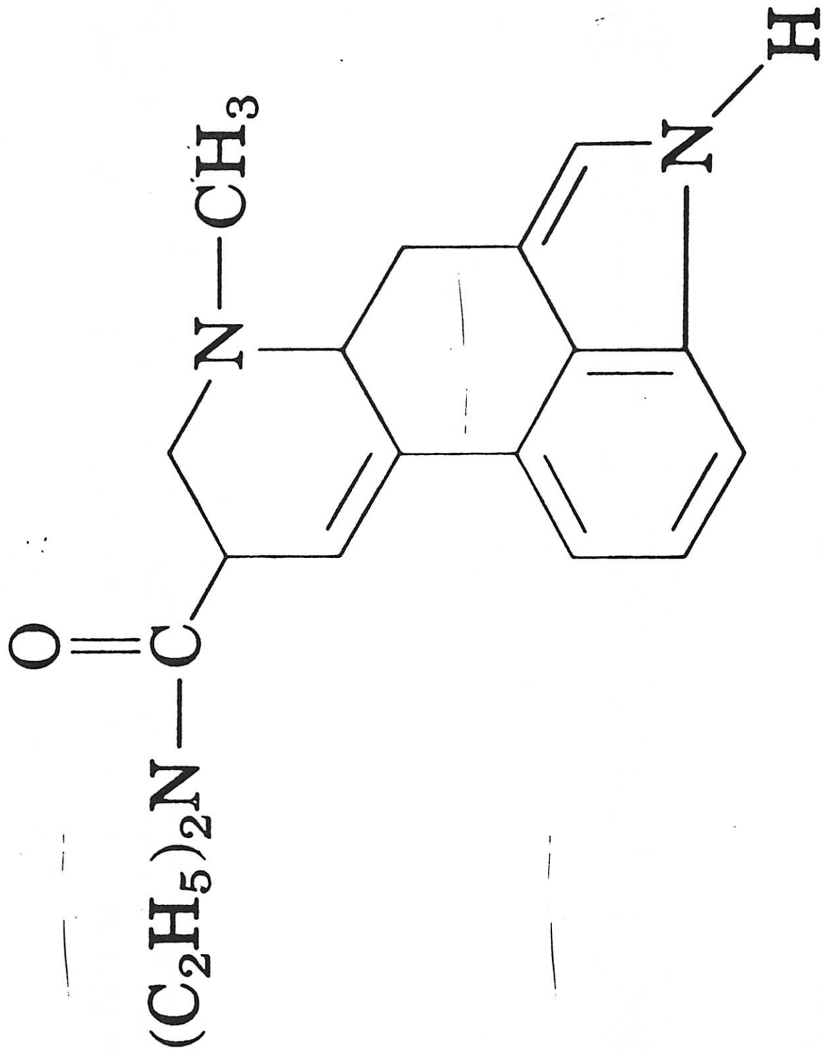
Lysergic acid diethylamide
