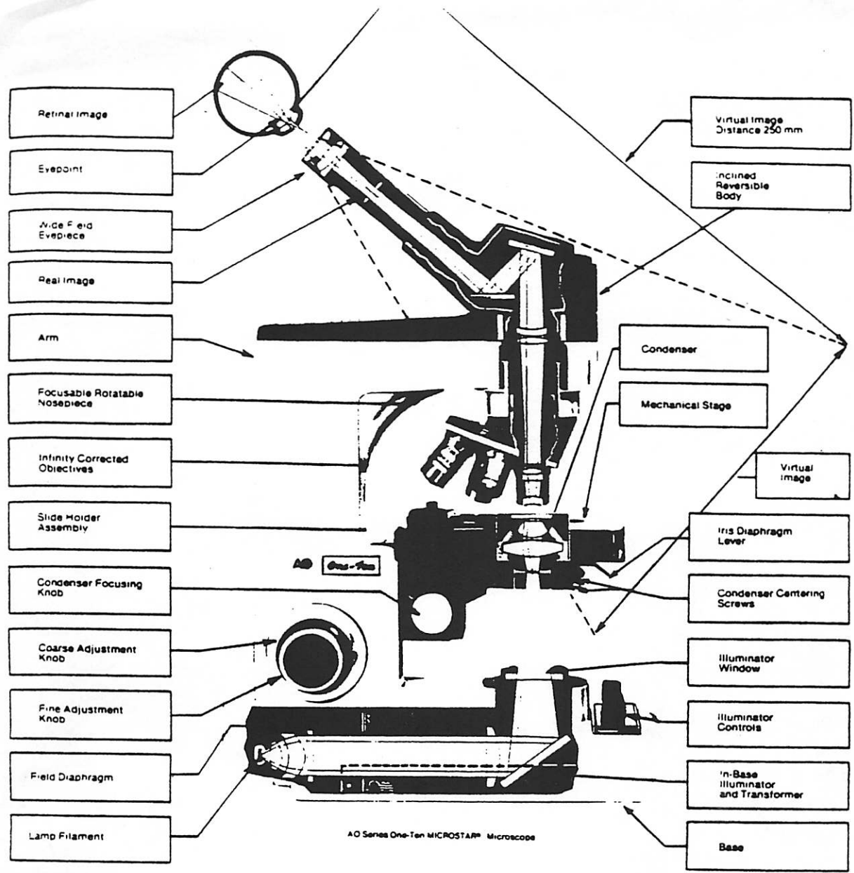
Figure 24.18. The ordinary bright-field light microscope. (Courtesy of American Optical Corporation)
