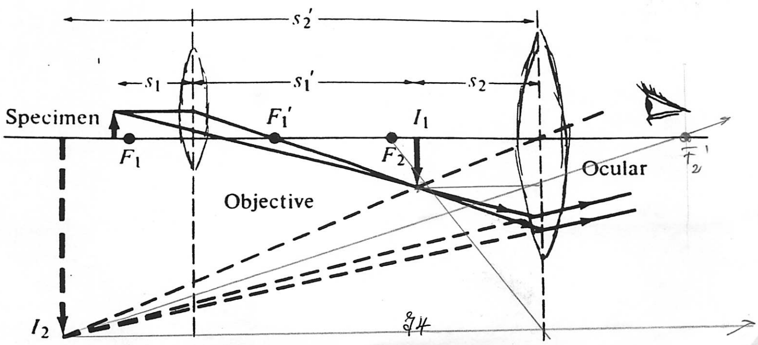
Figure 24.18. The ordinary bright-field light microscope. (Courtesy of American Optical Corporation)
