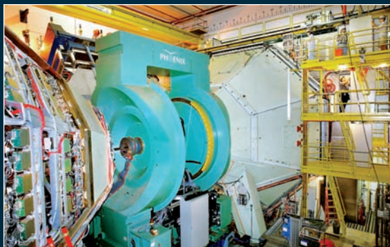
PHENIX experiment (shown here in partial disassembly during maintenance) searches for specific particles produced very early in the mini bangs.
