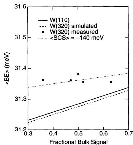
FIG. 4. Centroid ( \langle BE \rangle ) vs bulk fractional signal for theoretical and measured W spectra. The solid line is from (simulated) W(110), the dashed line is from simulated W(320), the filled circles are from measured W(320) spectra, and the dotted line is for an average SCS of -140 meV.
