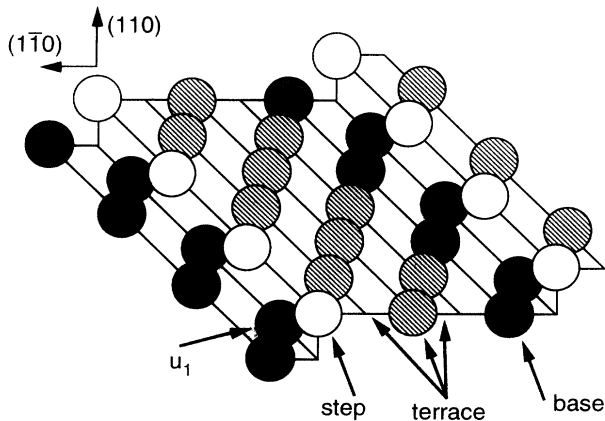
FIG. 1. Model of a bulk-truncated bcc(320) surface.
