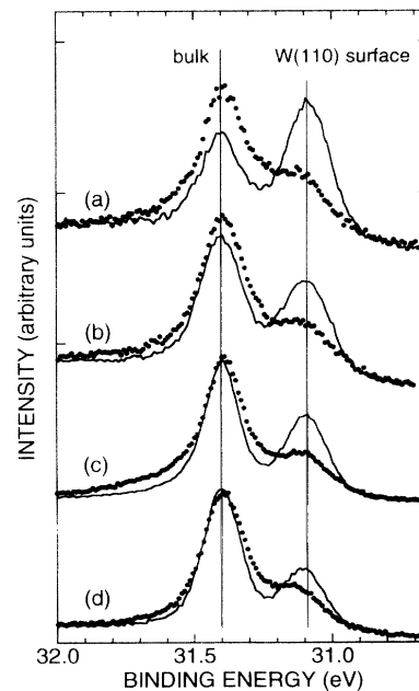
FIG. 2. Back-to-back data-set pairs taken on W(110) (solid lines) and W(320) (filled circles). The bulk and W(110) surface-atom BE's are marked with the vertical lines. (a) and (b) Photon energy = 60 eV, two different scattering geometries. (c) Photon energy = 90 eV. (d) Photon energy = 65 eV.
