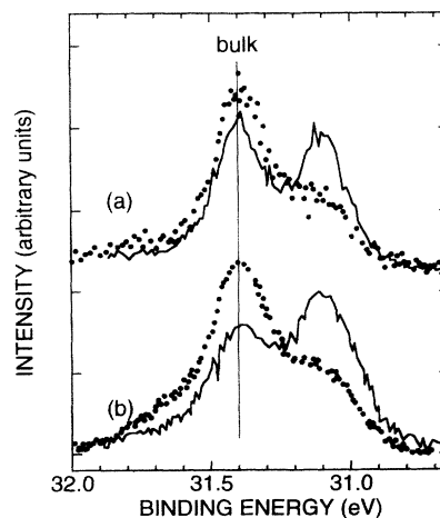
FIG. 8. Same data as in Fig. 7 except W(320) spectra have been shifted up in BE by 110 meV ( a ) (Ref. 6) and 300 meV ( b ) (Ref. 5).
