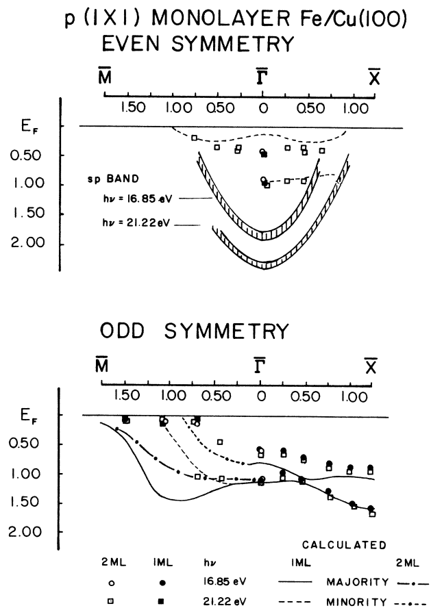
FIG. 2. Two-dimensional electronic structure of p(1 \times 1) Fe on Cu(100). The two broad curves indicate the regions of binding energy and k_{||} where a prominent structure resulting from the Cu sp band is observed. Light solid and dashed curves represent calculated (Ref. 5) surface Fe bands having over 50% surface character. Data are represented by empty (two-monolayer films) and solid (one-monolayer films) circles ( h\nu = 16.85 eV) and rectangles ( h\nu = 21.11 eV).
