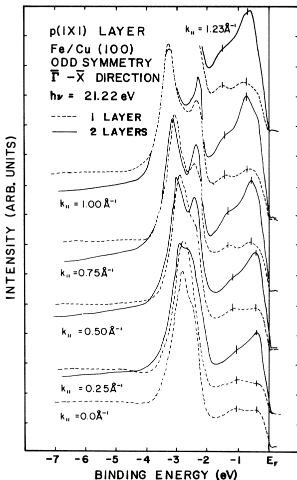
FIG. 1. Angle-resolved photoemission spectra for one- and two-layer p(1 \times 1) Fe films on Cu(100). Values of k_{||} correspond to the \bar{\Gamma} - \bar{X} direction of the two-dimensional Brillouin zone.
