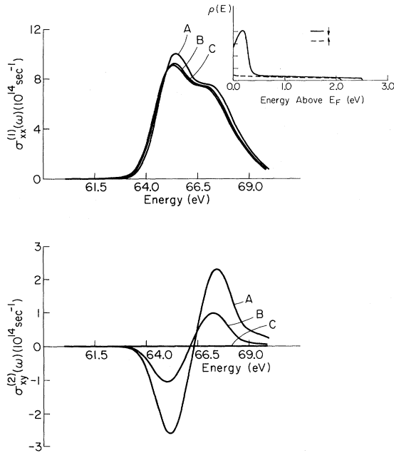
FIG. 4. Optical and magneto-optical absorption of the M_{23} edge in nickel. Insert: density-of-states model for unfilled final d states. A Gaussian with a 1.5-eV-wide full width at half-maximum was used to broaden the spectra. The curves A correspond to full magnetic moment ( T=0 ). Curves B and C correspond to Stoner model predictions for successively higher temperatures, T=T_c , for curve C .
