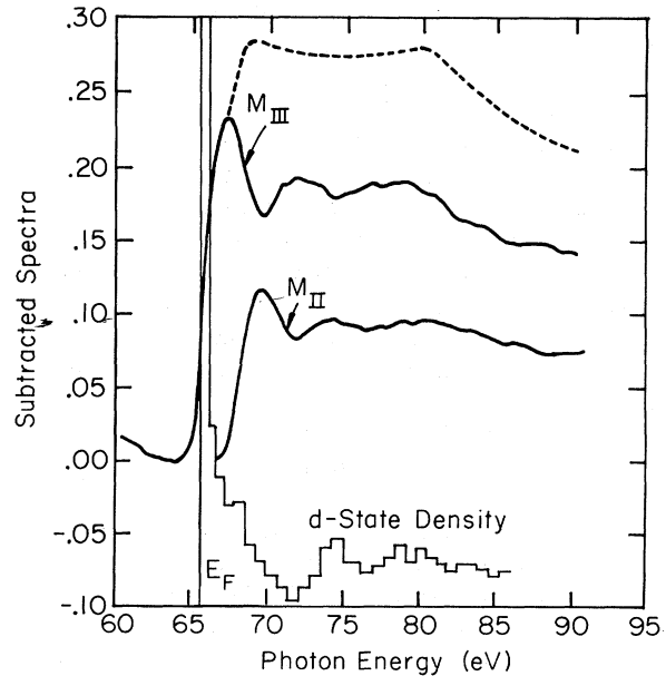
FIG. 2. Measured M spectrum components of Ni compared with the component density of d states above E_F (Ref. 26).
