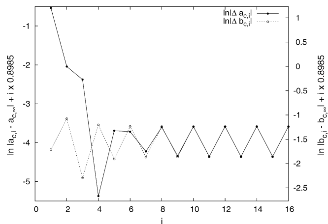
Fig. 1. 2-cycle of a_{c,i} and b_{c,i} differences in approximating the critical shearless torus \omega = \sqrt{2} - 1 by noble tori T_i . The average (negative) slope has been added to the data.
