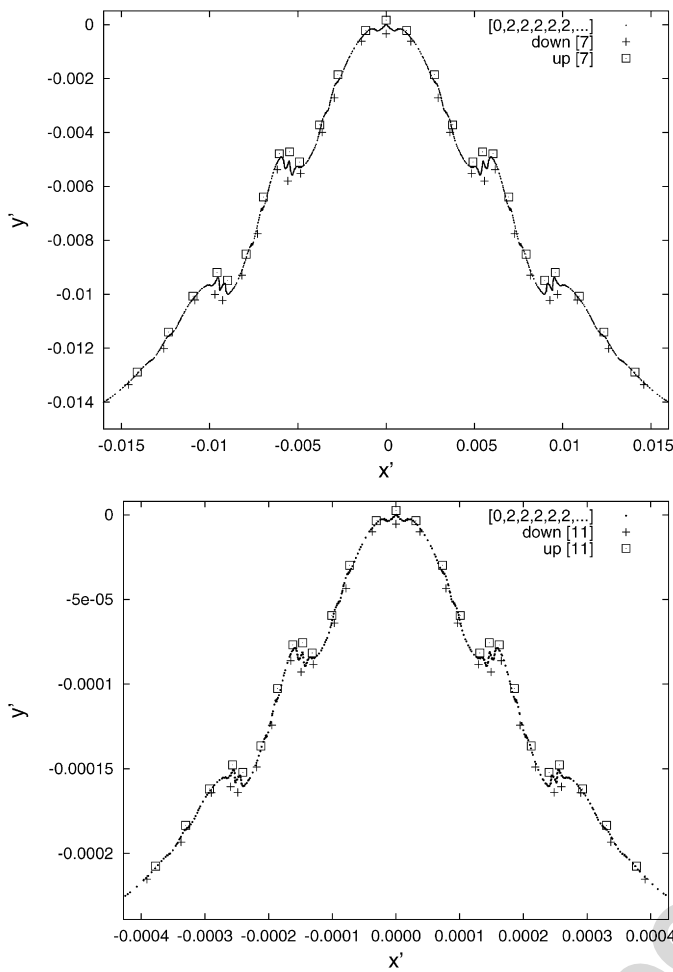
Fig. 4. Two levels of magnification in symmetry line coordinates (x', y') of the \omega = \sqrt{2} - 1 torus at breakup. Also shown are the nearby up and down orbits of the [7]th (top) and [11]th (bottom) continued fraction convergents.
