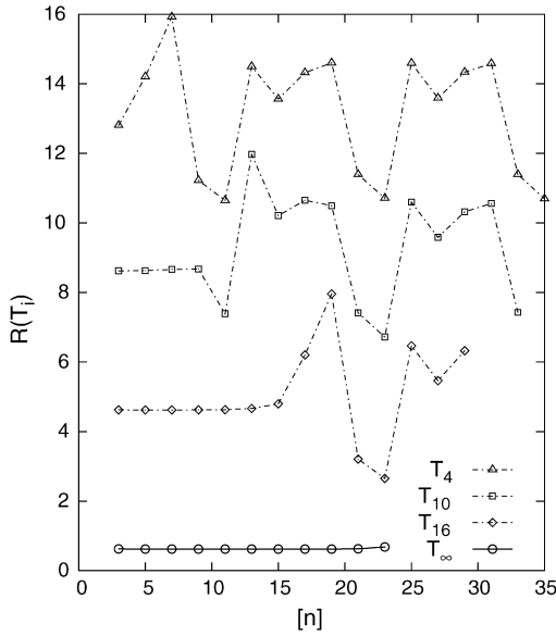
Fig. 2. Residue behavior at the shearless T_i torus breakup for down orbits on s_1 . For clarity the residues of the tori have been shifted upward by 4. (See text for definition of T_\infty .)
