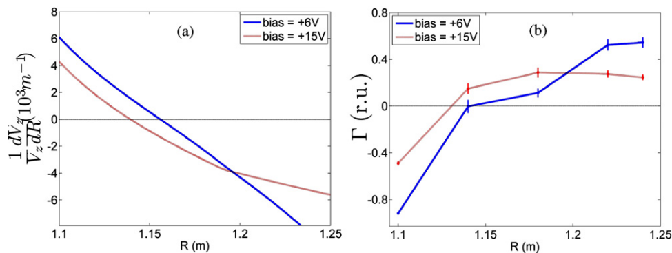
Figure 8. (a) Shear radial profile in Helimak discharges for two bias voltages. (b) Radial profile of turbulence-driven particle flux in Helimak for two bias voltages
