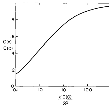
FIG. 4. Asymptotic soliton amplitude versus initial amplitude.
