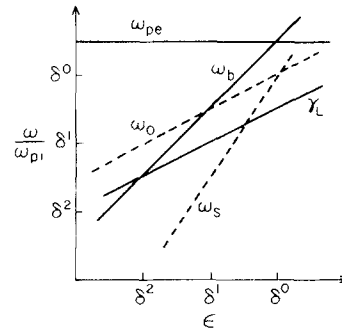
FIG. 1. Plot of relevant characteristic frequencies versus \epsilon \equiv e\Phi/T_e .
