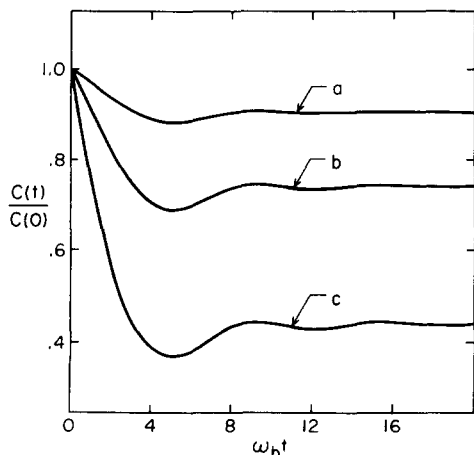
FIG. 3. Plots of c(t)/c(0) versus time. (a) \gamma_L/\omega_b = 0.057 , (b) \gamma_L/\omega_b = 0.183 , and (c) \gamma_L/\omega_b = 0.57 . Note that \omega_b depends on c(0) .
