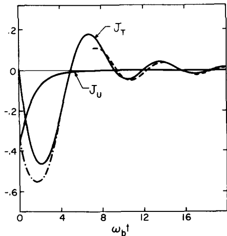
FIG. 2. Plots of trapped ( J_T ) and untrapped ( J_u ) contributions to the generalized damping coefficient \gamma . J_u + J_T is indicated by dash-dot. Dashed curve indicates the asymptotic behavior of J_T .
